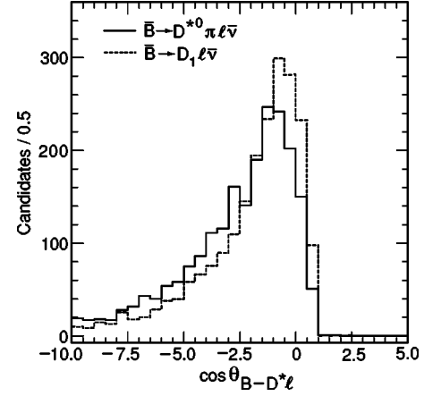
FIG. 20. The \cos \theta_{B-D^*\ell} distribution of \bar{B} \rightarrow D^{*0}\pi\ell\bar{\nu} (solid histogram) and \bar{B} \rightarrow D_1\ell\bar{\nu} (dashed histogram) decays contributing to the D^*X\ell\bar{\nu} sample for D^{*0}\ell\bar{\nu} . The histograms are normalized to equal area.
